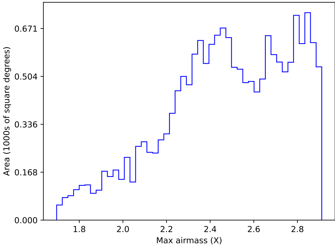
roll_uniform_early_half_mjdp0_v3.4_10yrs WFD i band: Max airmass
