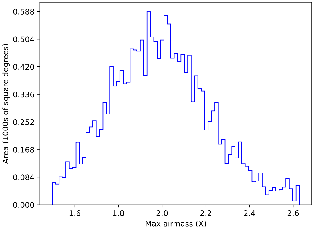
roll_uniform_early_half_mjdp0_v3.4_10yrs WFD g band: Max airmass
