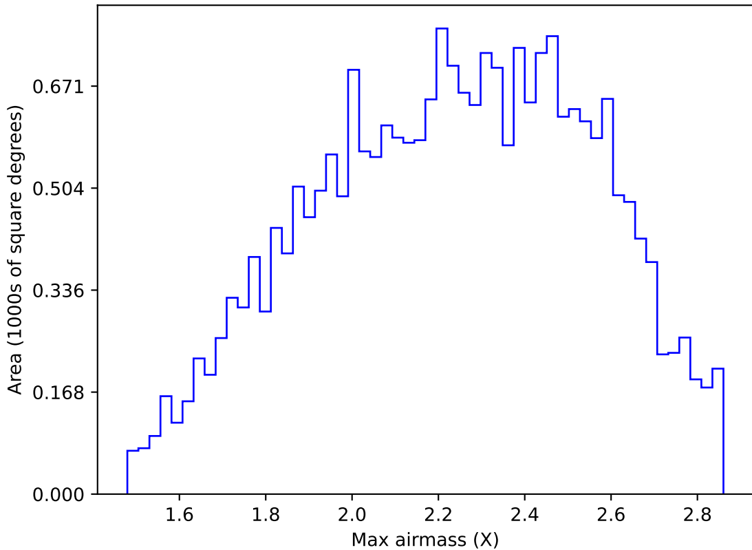
roll_uniform_early_half_mjdp0_v3.4_10yrs All sky y band: Max airmass
