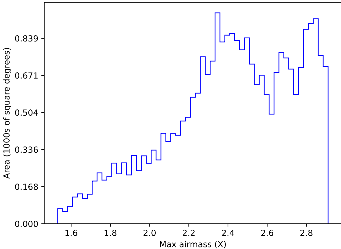
roll_uniform_early_half_mjdp0_v3.4_10yrs All sky i band: Max airmass
