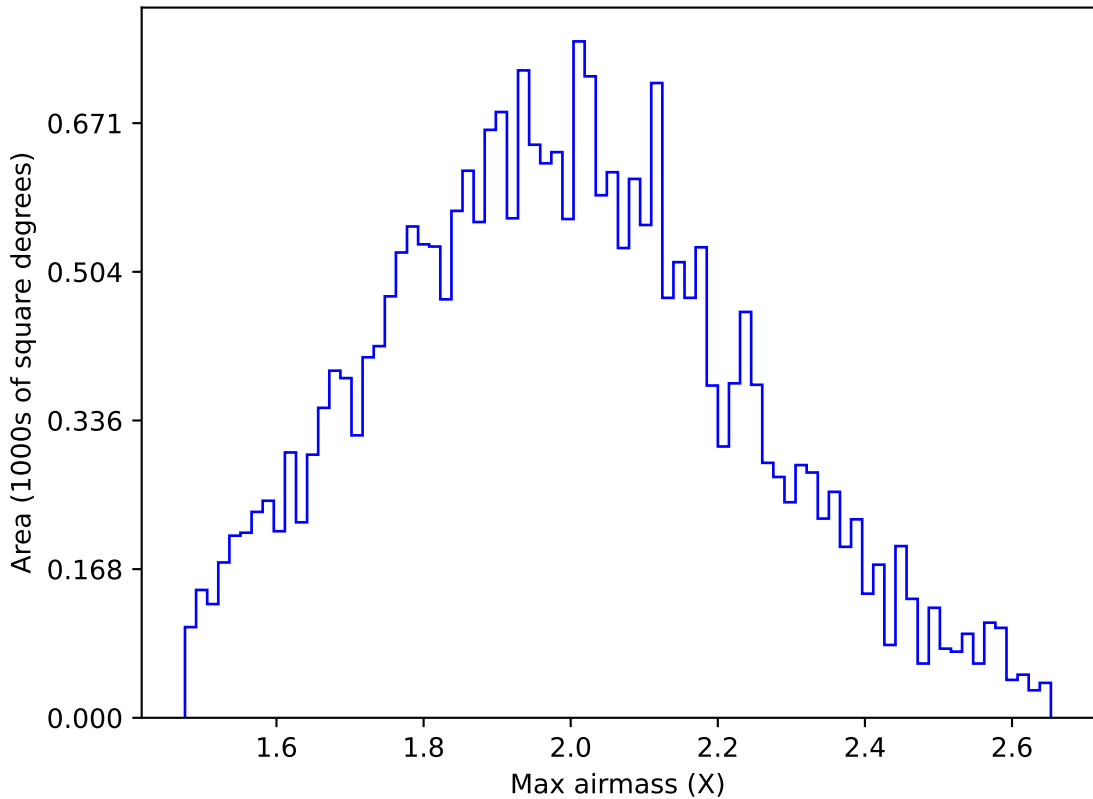
roll_uniform_early_half_mjdp0_v3.4_10yrs All sky g band: Max airmass
