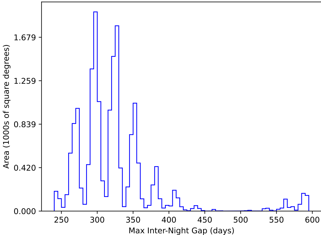
roll_uniform_early_half_mjdp0_v3.4_10yrs WFD y band: Max Inter-Night Gap
