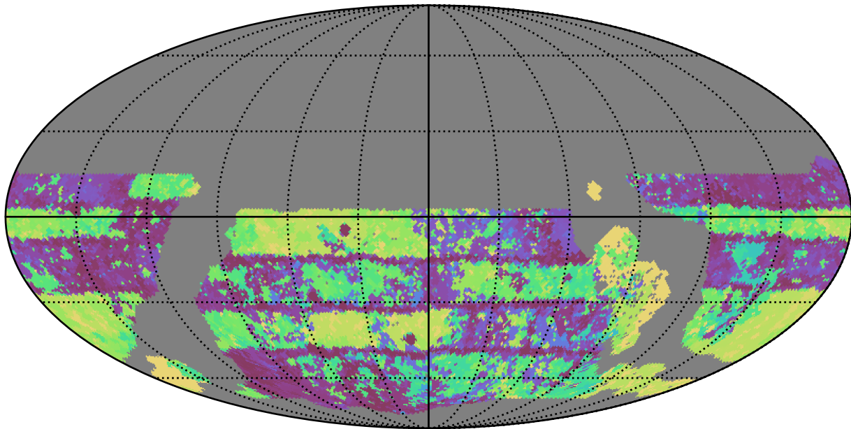
roll_uniform_early_half_mjdp0_v3.4_10yrs WFD u band: Max Inter-Night Gap
