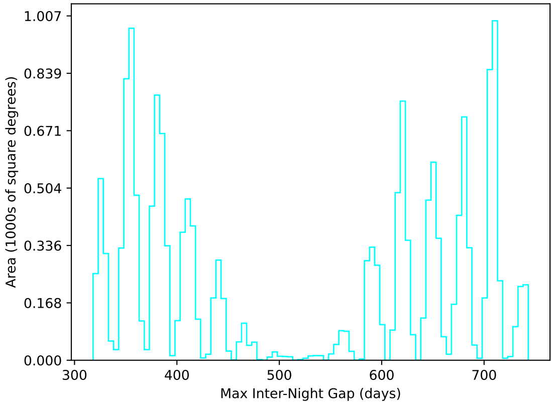
roll_uniform_early_half_mjdp0_v3.4_10yrs WFD u band: Max Inter-Night Gap
