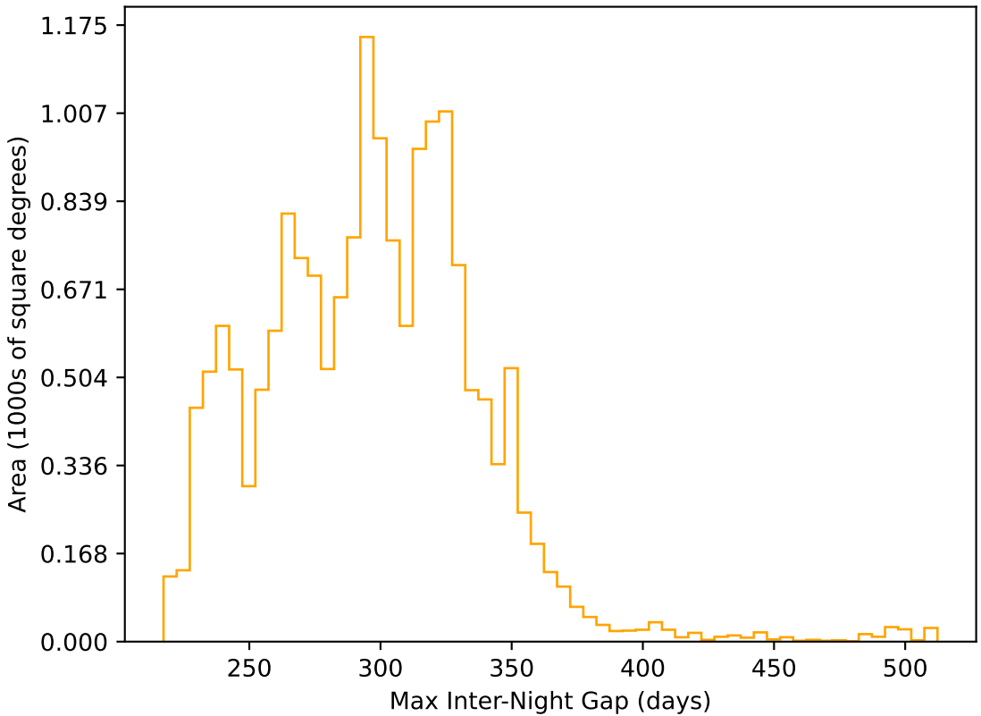
roll_uniform_early_half_mjdp0_v3.4_10yrs WFD r band: Max Inter-Night Gap
