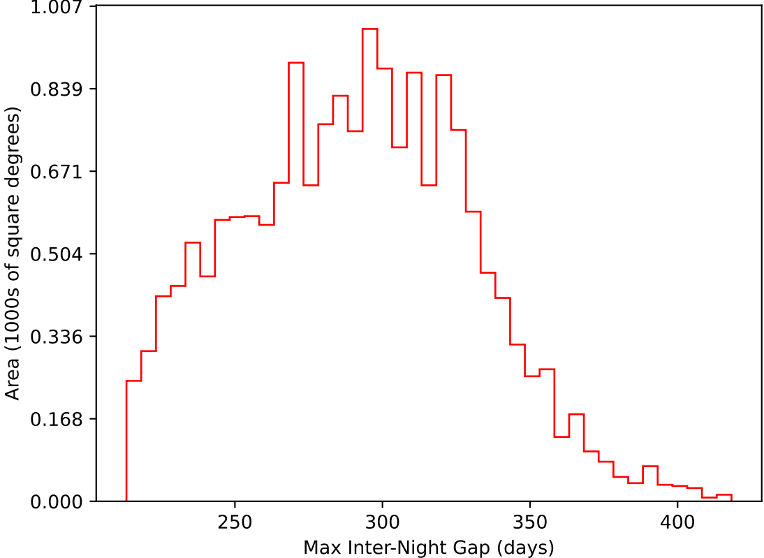
roll_uniform_early_half_mjdp0_v3.4_10yrs WFD i band: Max Inter-Night Gap
