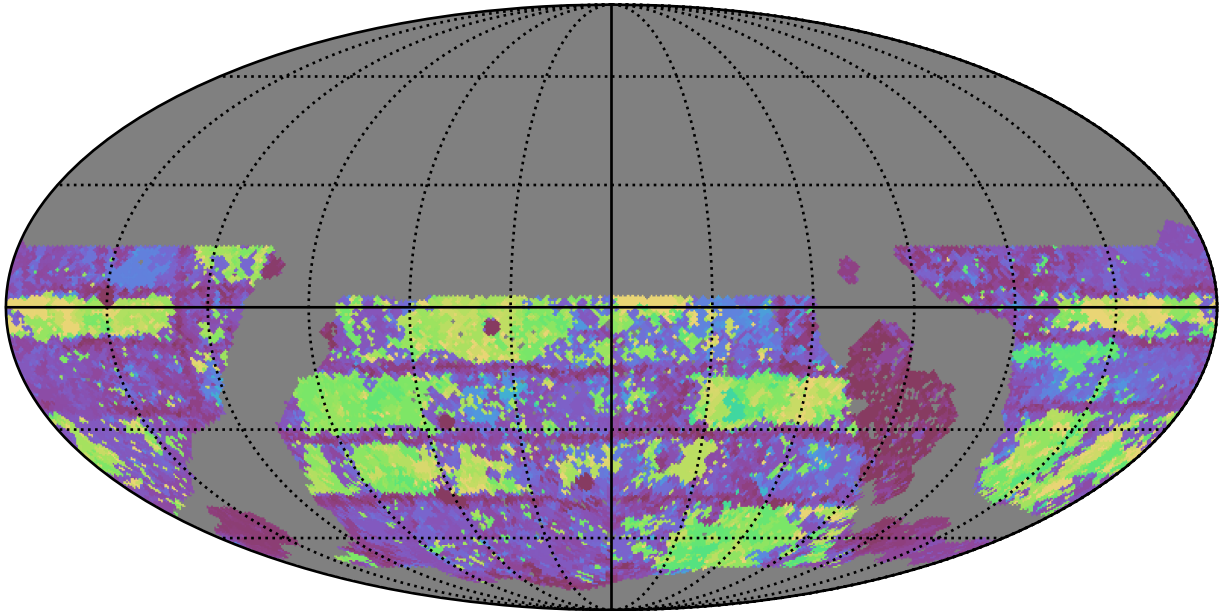
roll_uniform_early_half_mjdp0_v3.4_10yrs WFD g band: Max Inter-Night Gap
