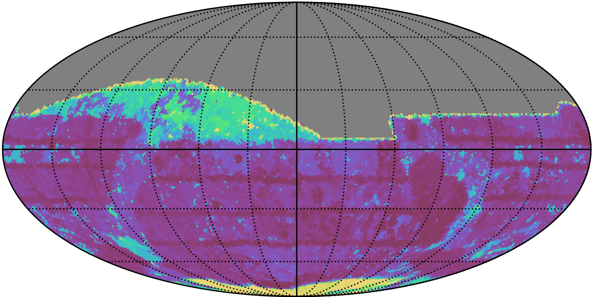
roll_uniform_early_half_mjdp0_v3.4_10yrs All sky z band: Max Inter-Night Gap
