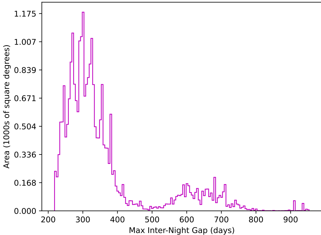
roll_uniform_early_half_mjdp0_v3.4_10yrs All sky z band: Max Inter-Night Gap
