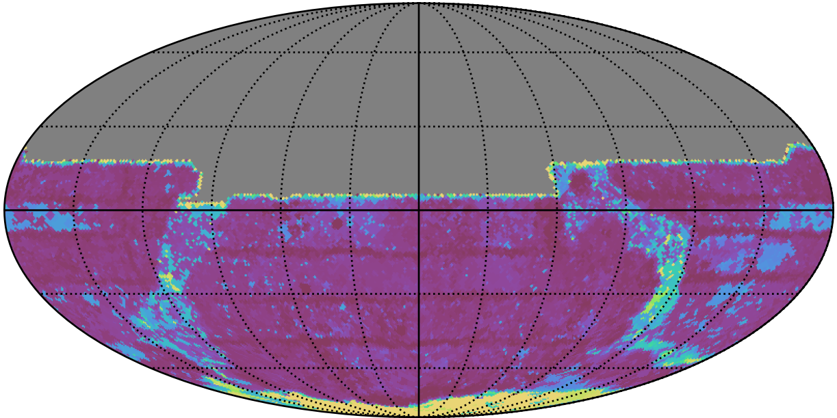
roll_uniform_early_half_mjdp0_v3.4_10yrs All sky y band: Max Inter-Night Gap
