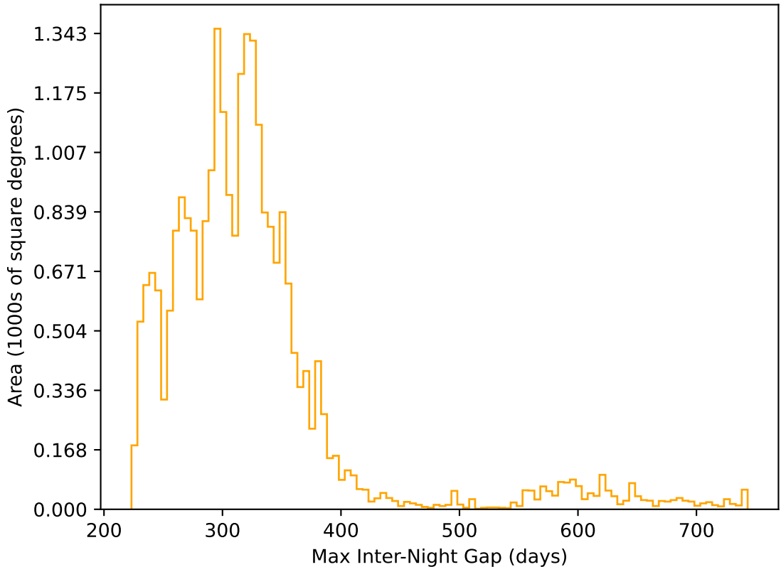
roll_uniform_early_half_mjdp0_v3.4_10yrs All sky r band: Max Inter-Night Gap
