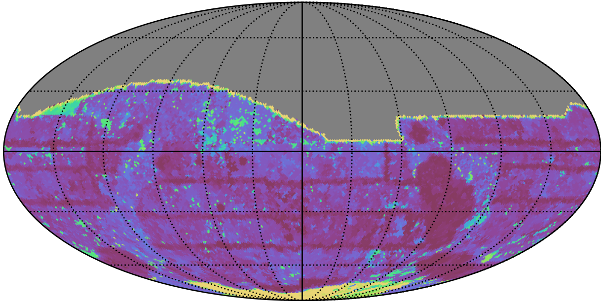
roll_uniform_early_half_mjdp0_v3.4_10yrs All sky i band: Max Inter-Night Gap
