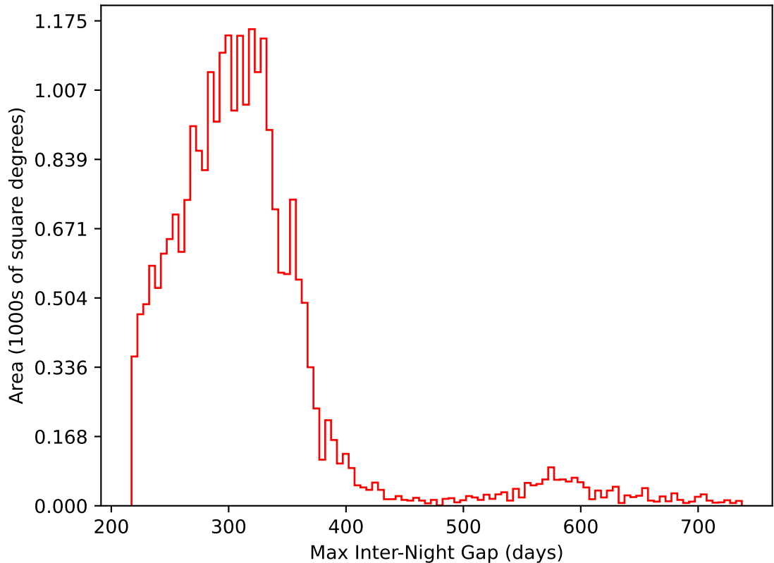
roll_uniform_early_half_mjdp0_v3.4_10yrs All sky i band: Max Inter-Night Gap
