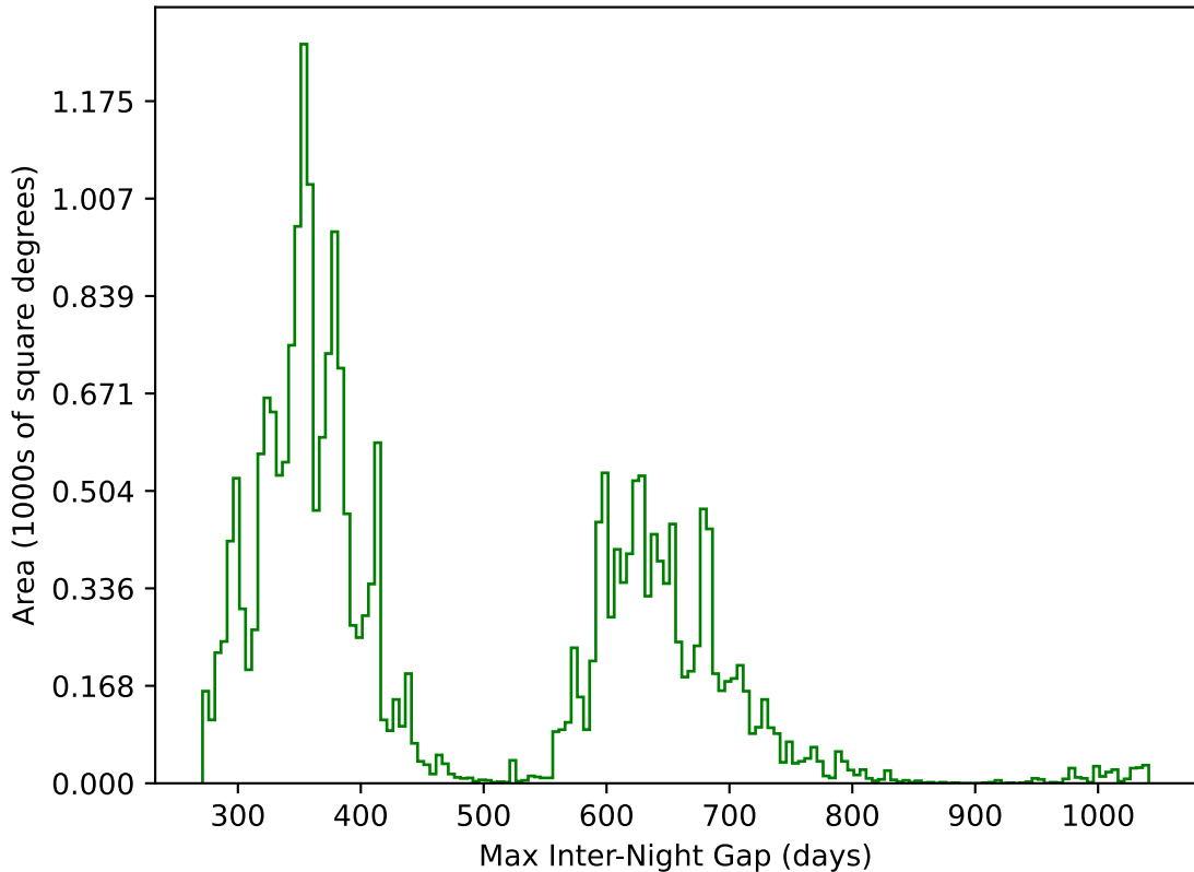
roll_uniform_early_half_mjdp0_v3.4_10yrs All sky g band: Max Inter-Night Gap
