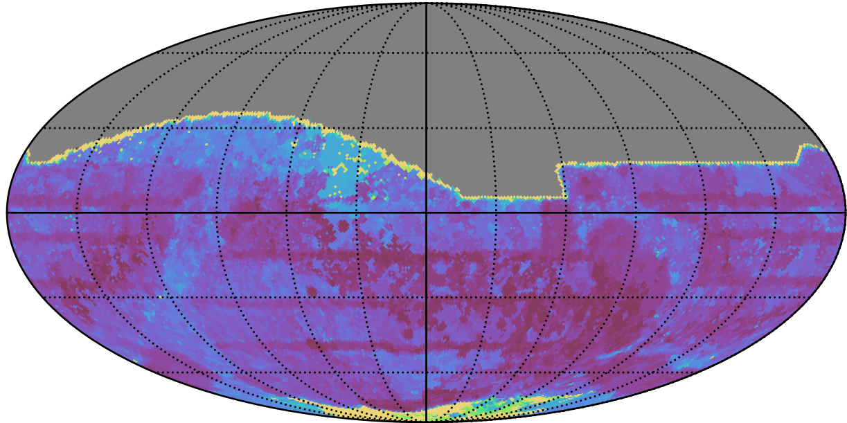
roll_uniform_early_half_mjdp0_v3.4_10yrs All sky all bands: Max Inter-Night Gap
