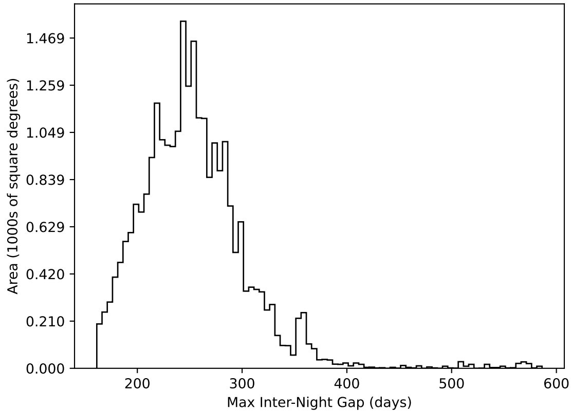
roll_uniform_early_half_mjdp0_v3.4_10yrs All sky all bands: Max Inter-Night Gap
