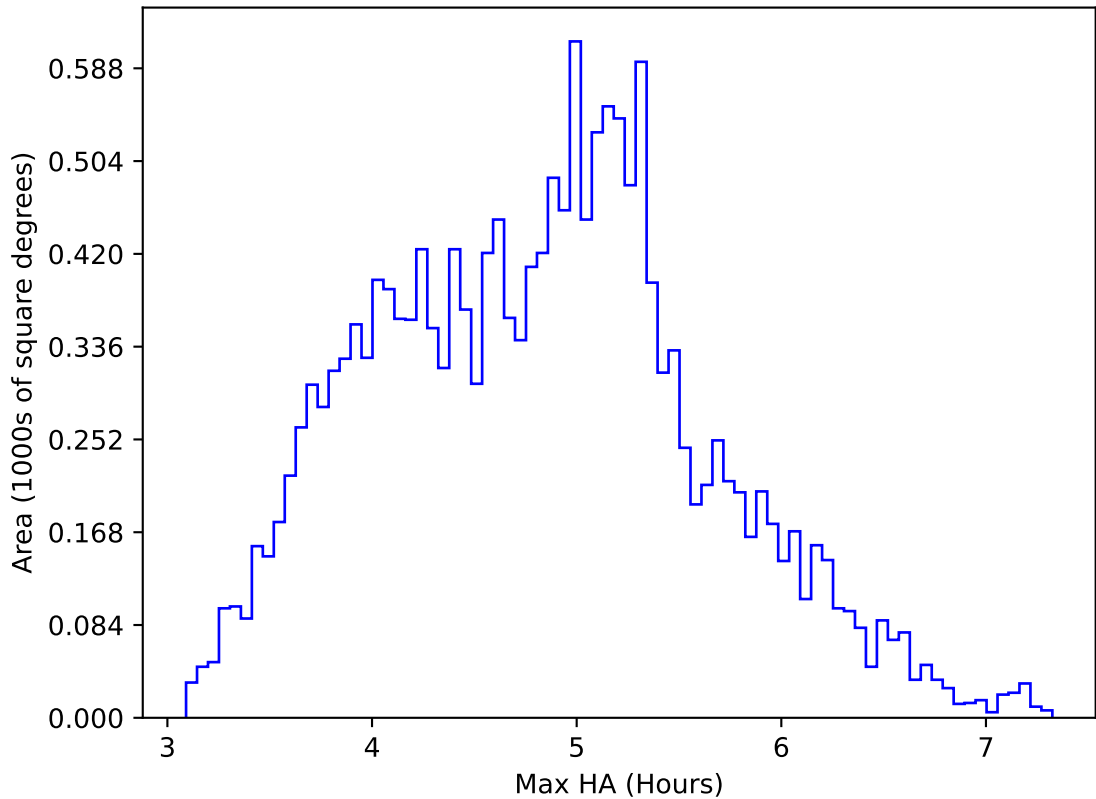
roll_uniform_early_half_mjdp0_v3.4_10yrs WFD z band: Max HA
