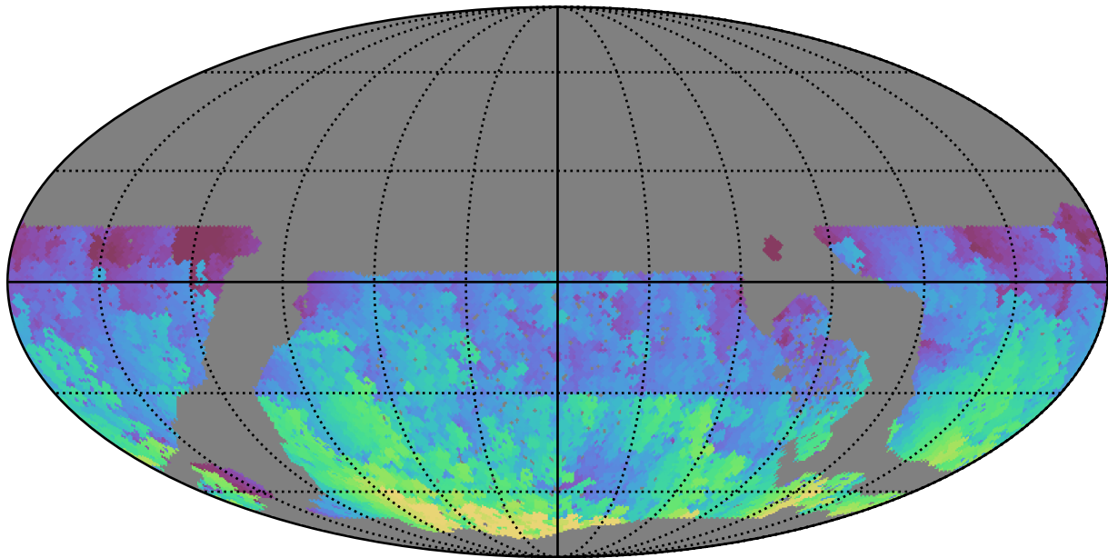
roll_uniform_early_half_mjdp0_v3.4_10yrs WFD u band: Max HA
