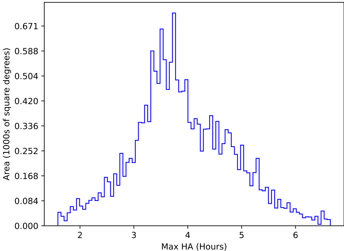
roll_uniform_early_half_mjdp0_v3.4_10yrs WFD u band: Max HA
