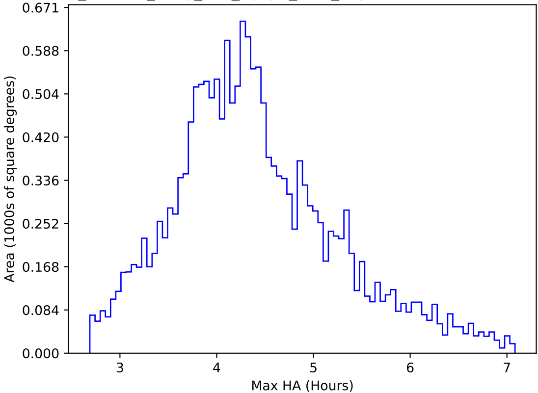
roll_uniform_early_half_mjdp0_v3.4_10yrs WFD r band: Max HA
