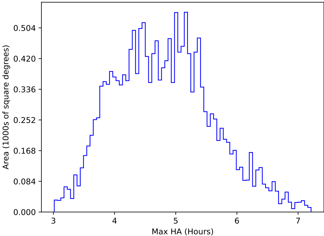
roll_uniform_early_half_mjdp0_v3.4_10yrs WFD i band: Max HA
