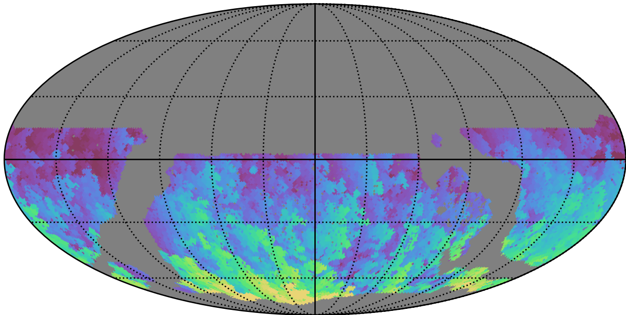
roll_uniform_early_half_mjdp0_v3.4_10yrs WFD g band: Max HA
