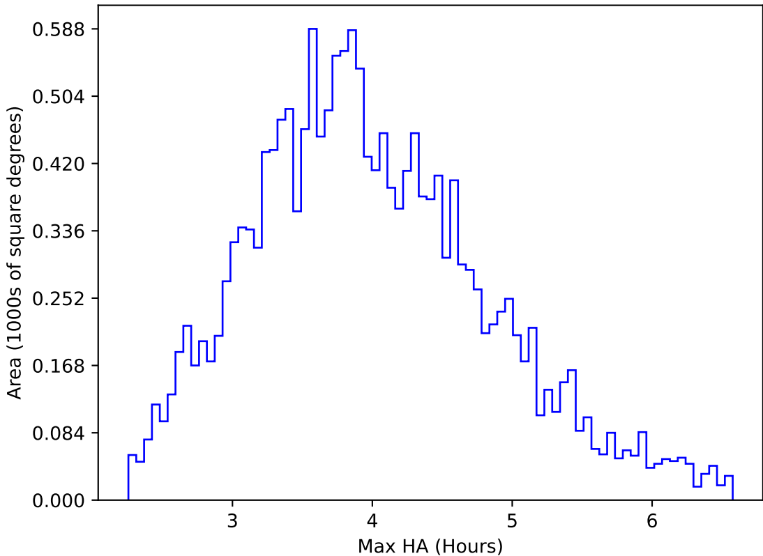
roll_uniform_early_half_mjdp0_v3.4_10yrs WFD g band: Max HA
