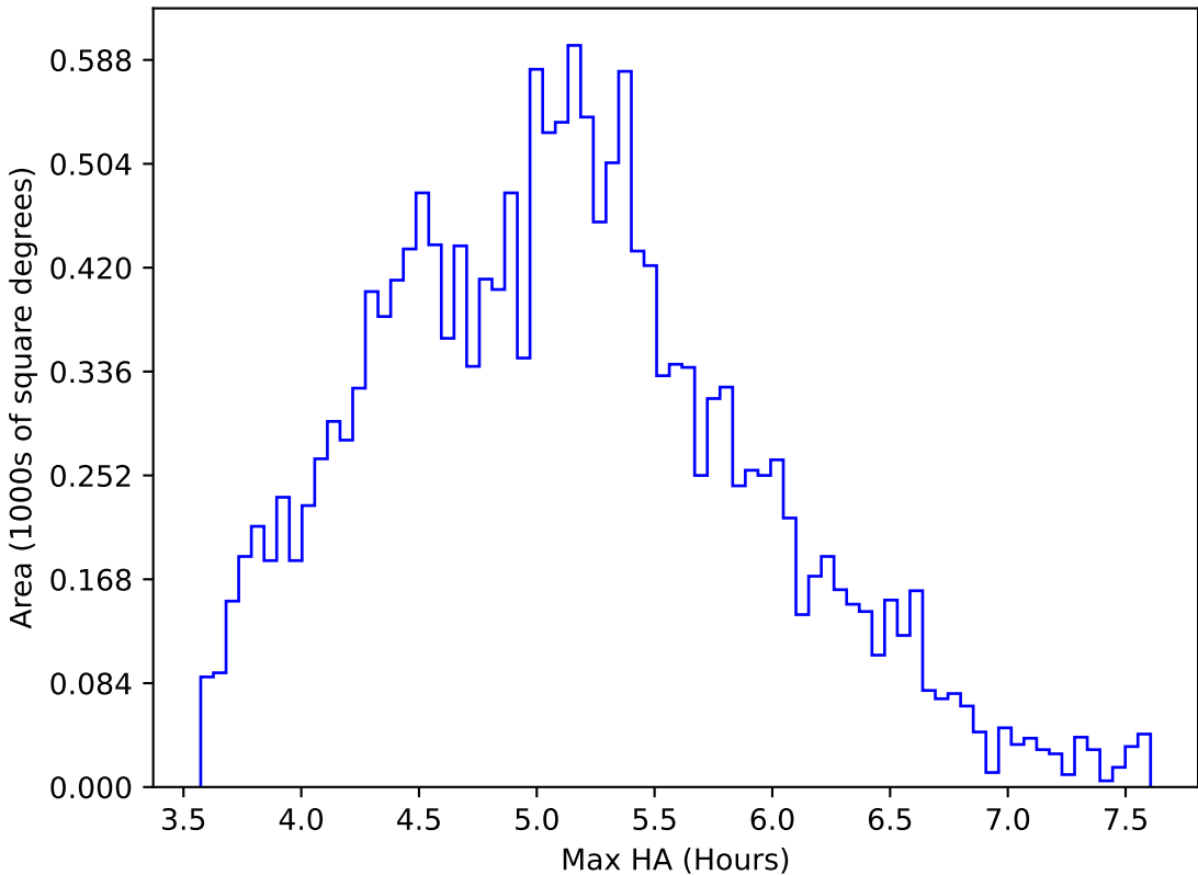
roll_uniform_early_half_mjdp0_v3.4_10yrs WFD all bands: Max HA
