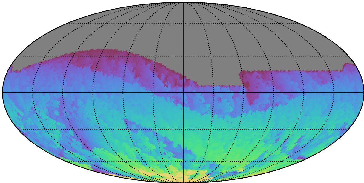
roll_uniform_early_half_mjdp0_v3.4_10yrs All sky z band: Max HA
