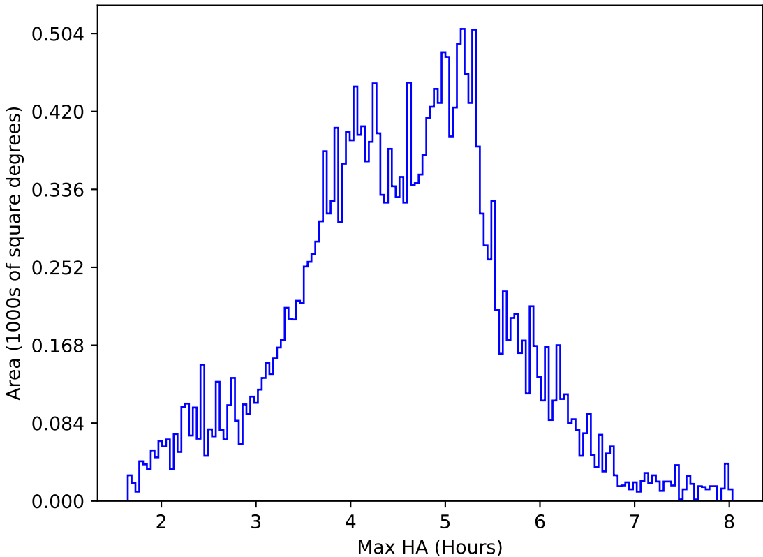
roll_uniform_early_half_mjdp0_v3.4_10yrs All sky z band: Max HA
