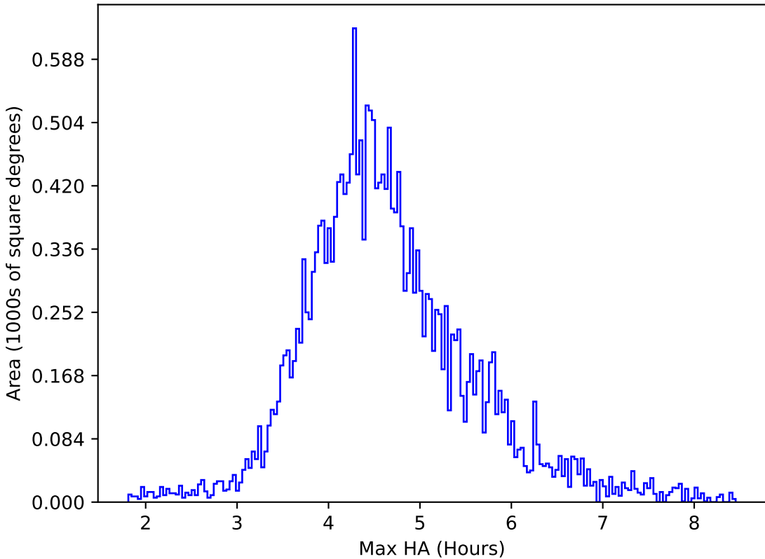
roll_uniform_early_half_mjdp0_v3.4_10yrs All sky y band: Max HA
