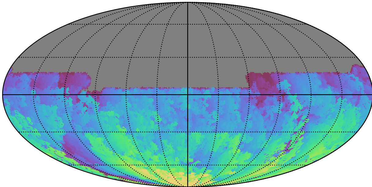
roll_uniform_early_half_mjdp0_v3.4_10yrs All sky u band: Max HA
