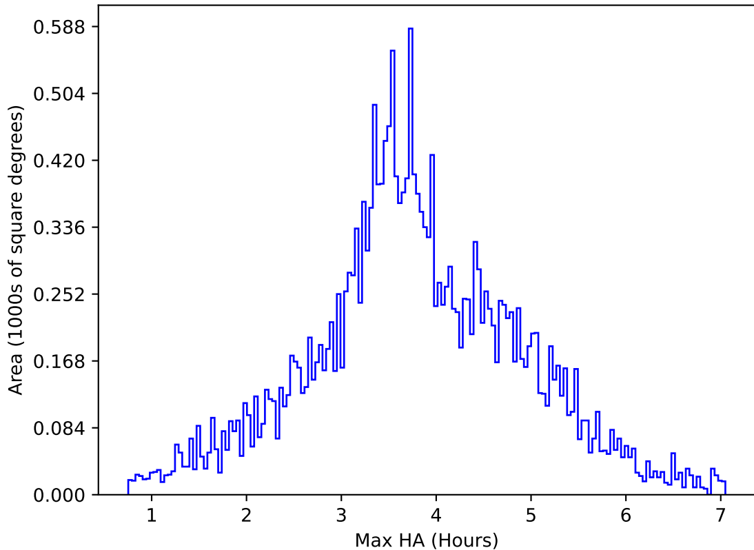
roll_uniform_early_half_mjdp0_v3.4_10yrs All sky u band: Max HA
