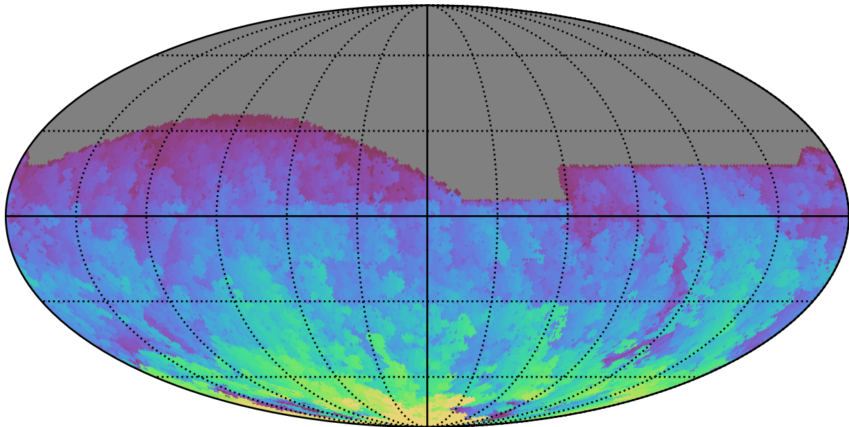
roll_uniform_early_half_mjdp0_v3.4_10yrs All sky r band: Max HA
