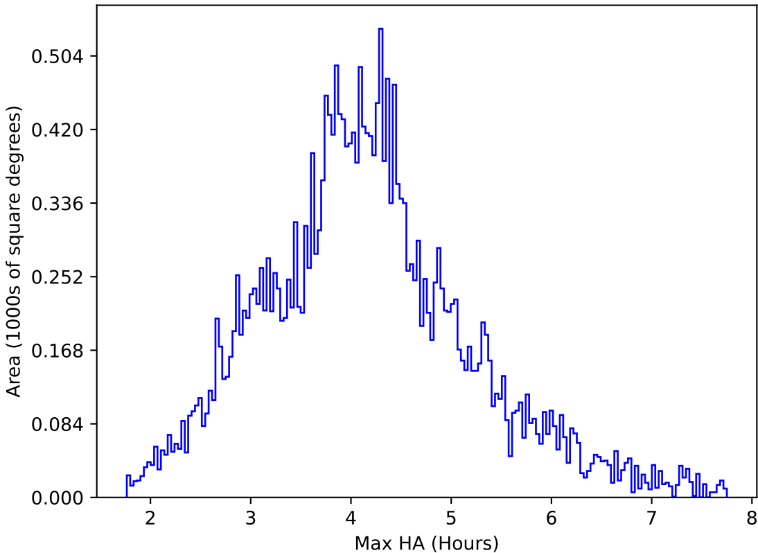
roll_uniform_early_half_mjdp0_v3.4_10yrs All sky r band: Max HA
