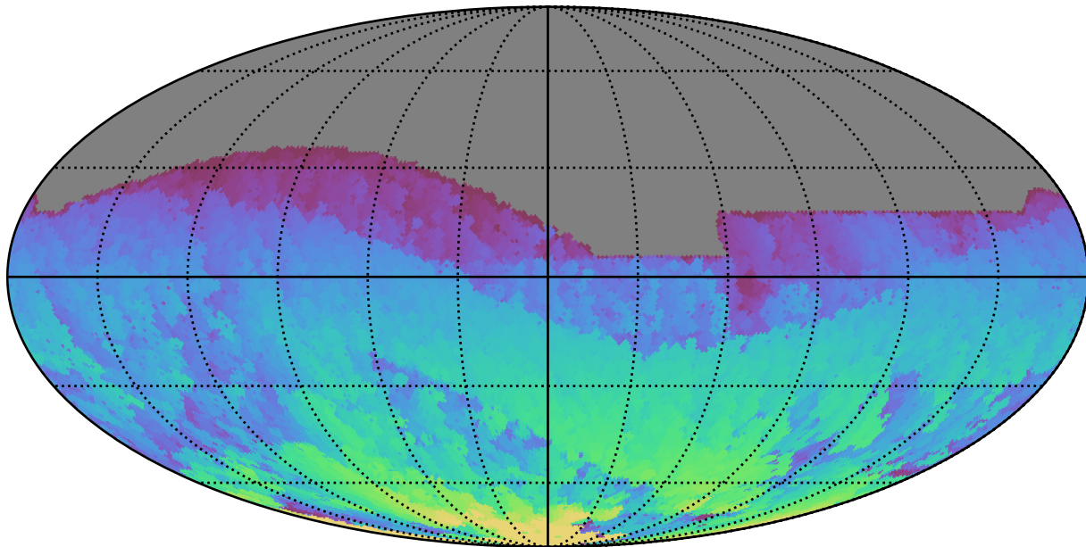
roll_uniform_early_half_mjdp0_v3.4_10yrs All sky i band: Max HA
