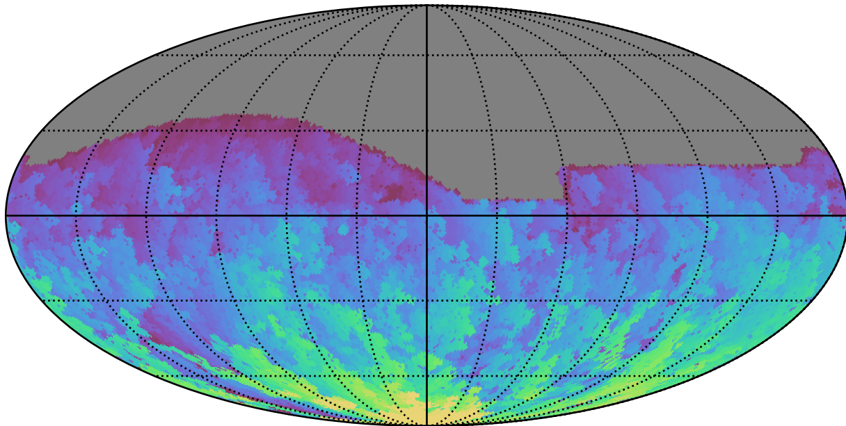
roll_uniform_early_half_mjdp0_v3.4_10yrs All sky g band: Max HA
