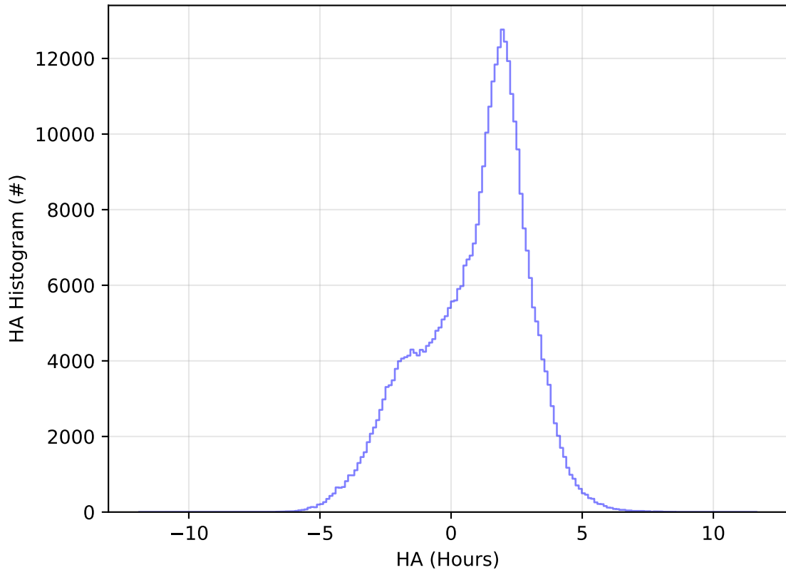
roll_uniform_early_half_mjdp0_v3.4_10yrs WFD y band: HA Histogram
