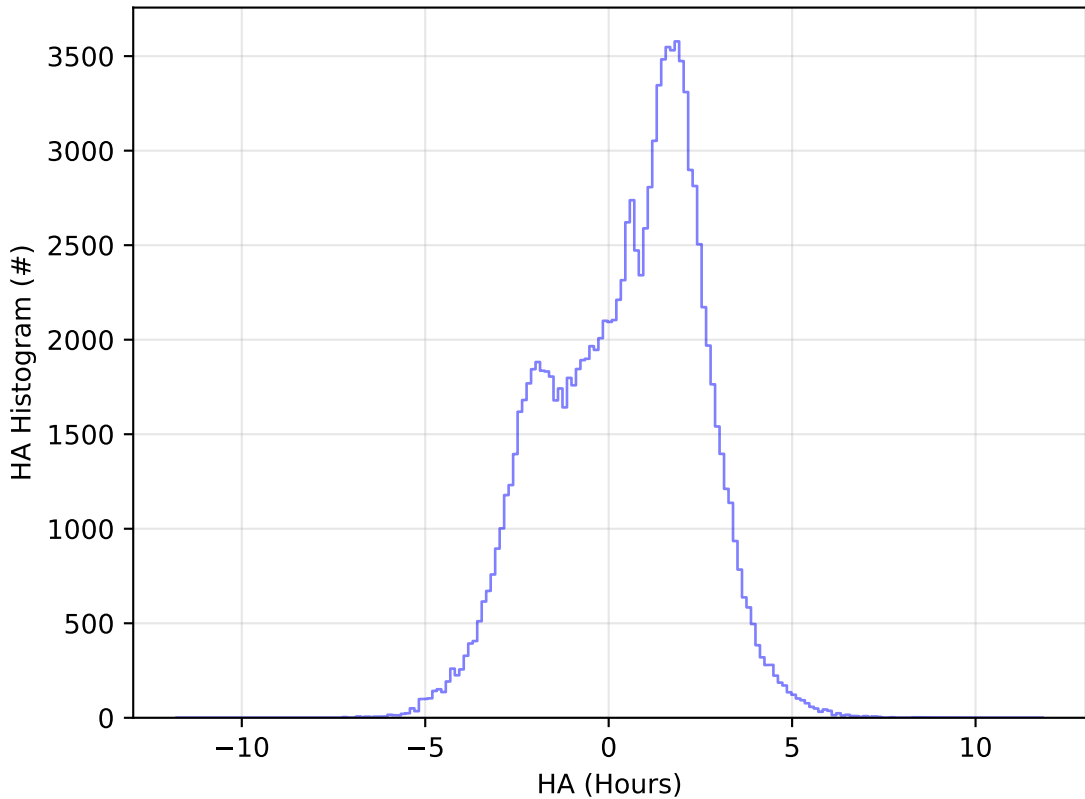
roll_uniform_early_half_mjdp0_v3.4_10yrs WFD u band: HA Histogram
