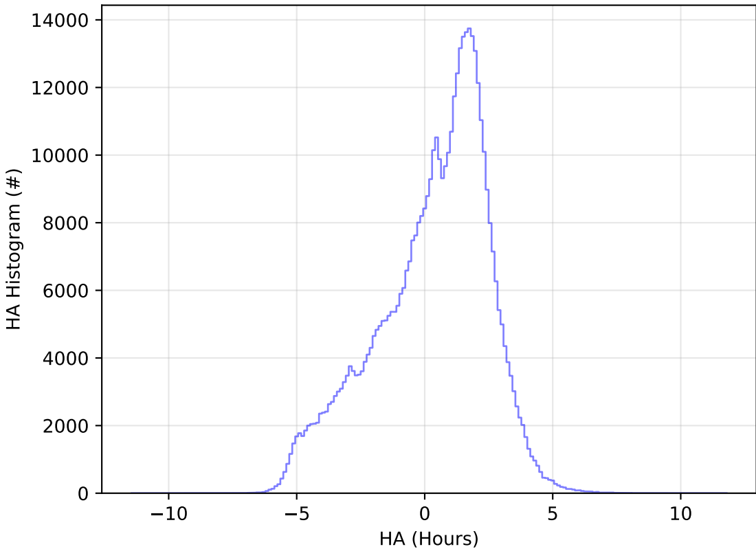
roll_uniform_early_half_mjdp0_v3.4_10yrs WFD r band: HA Histogram
