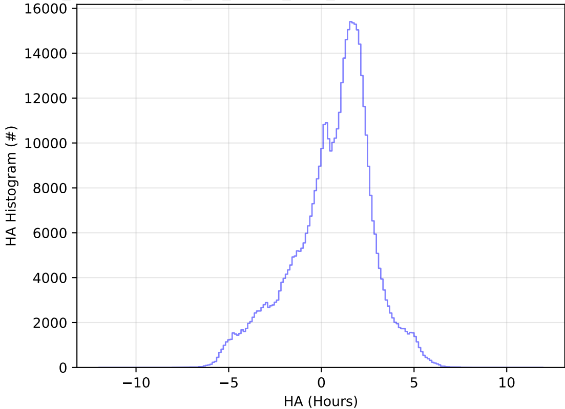
roll_uniform_early_half_mjdp0_v3.4_10yrs WFD i band: HA Histogram
