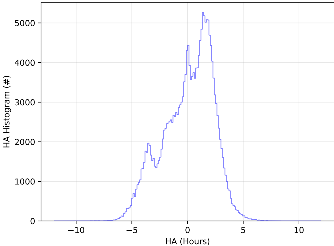
roll_uniform_early_half_mjdp0_v3.4_10yrs WFD g band: HA Histogram
