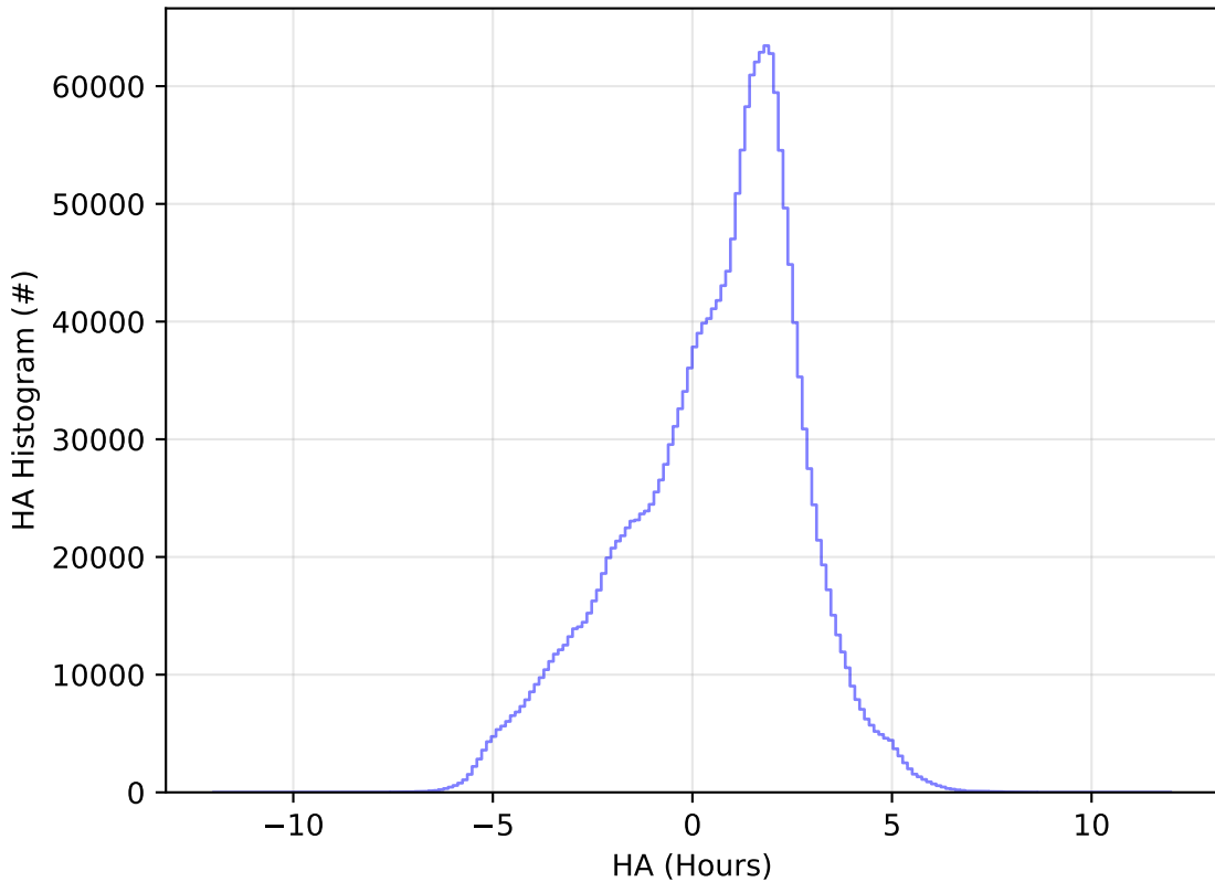
roll_uniform_early_half_mjdp0_v3.4_10yrs WFD all bands: HA Histogram
