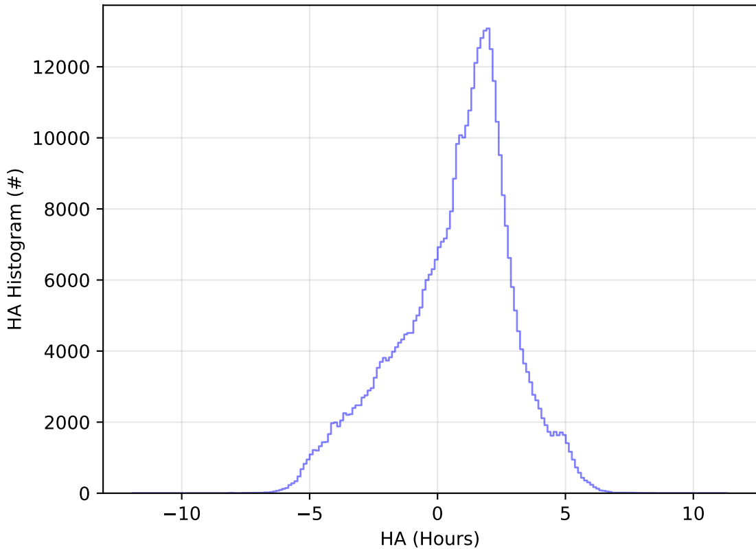
roll_uniform_early_half_mjdp0_v3.4_10yrs All sky z band: HA Histogram
