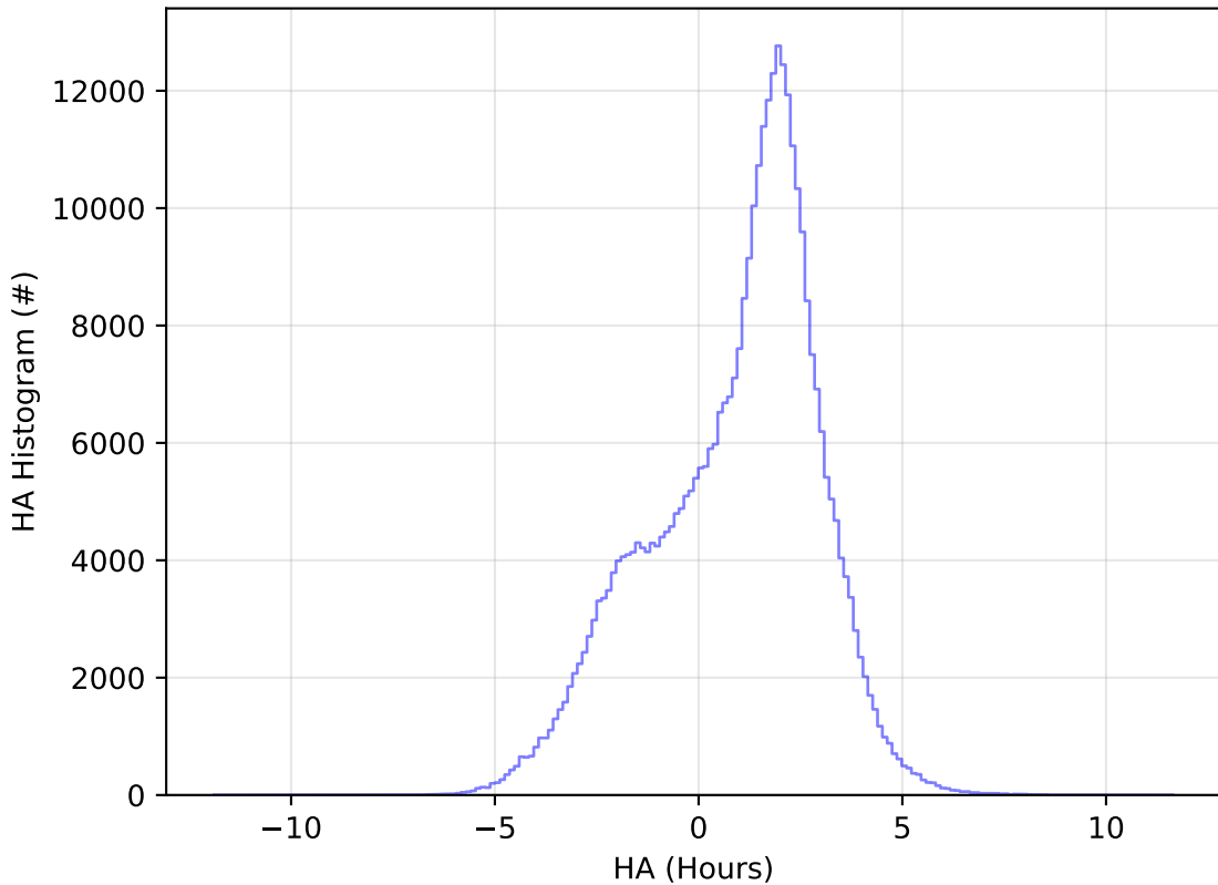
roll_uniform_early_half_mjdp0_v3.4_10yrs All sky y band: HA Histogram
