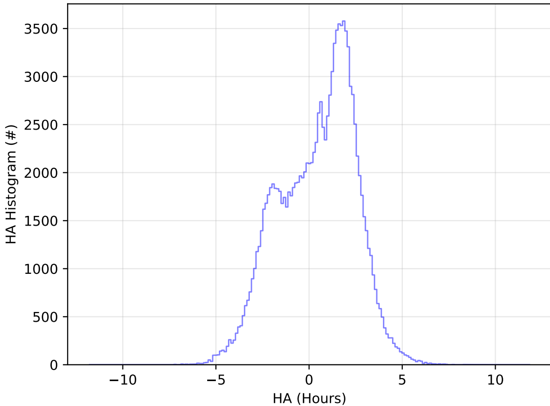
roll_uniform_early_half_mjdp0_v3.4_10yrs All sky u band: HA Histogram
