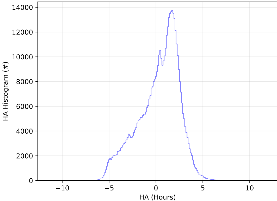
roll_uniform_early_half_mjdp0_v3.4_10yrs All sky r band: HA Histogram
