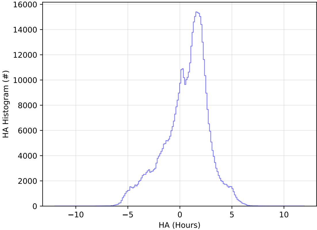
roll_uniform_early_half_mjdp0_v3.4_10yrs All sky i band: HA Histogram
