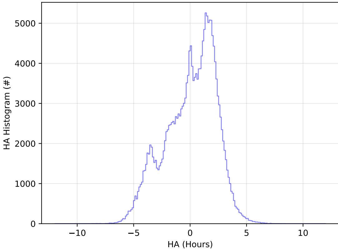
roll_uniform_early_half_mjdp0_v3.4_10yrs All sky g band: HA Histogram
