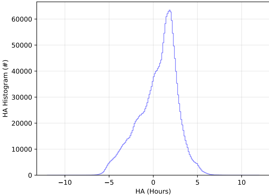
roll_uniform_early_half_mjdp0_v3.4_10yrs All sky all bands: HA Histogram
